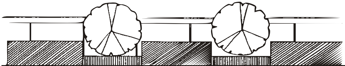
Figure 9-4: Existing Tree Crown - Proposed Awning Conflict Plan
