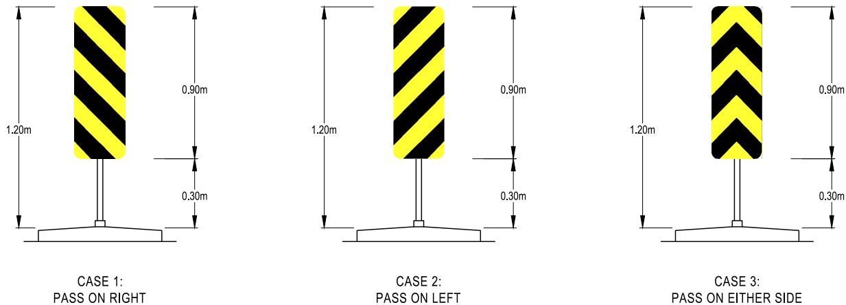
Figure 8-10: Object Marker Sign Placement
