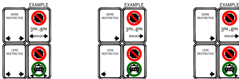
VERTICAL SIGN PLACEMENT ASSEMBLY
