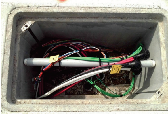
Figure 10-9: Street Lighting Junction Box Example
