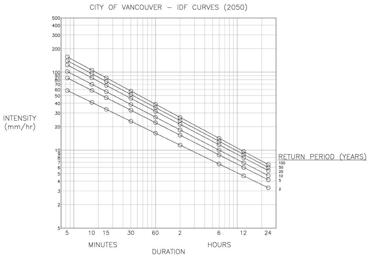
Figure 5-2: 2050 IDF Curve
