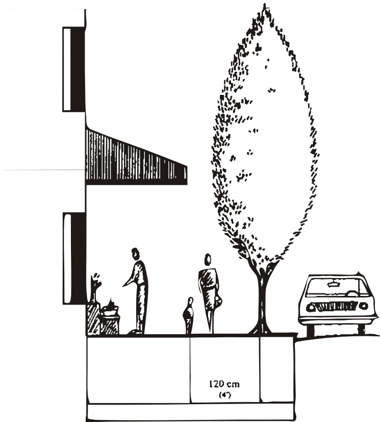
Figure 9-5: Narrow Boulevard Columnar Tree Awning Section
